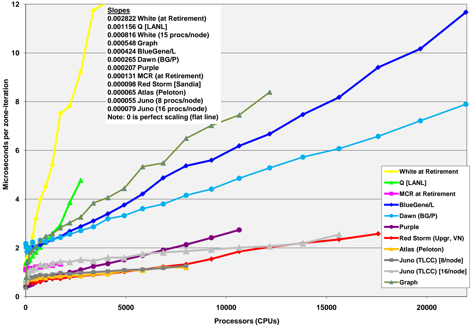
Weak Scaling - Historic 3D Radiation problem's average zone-iteration grind time per machine
